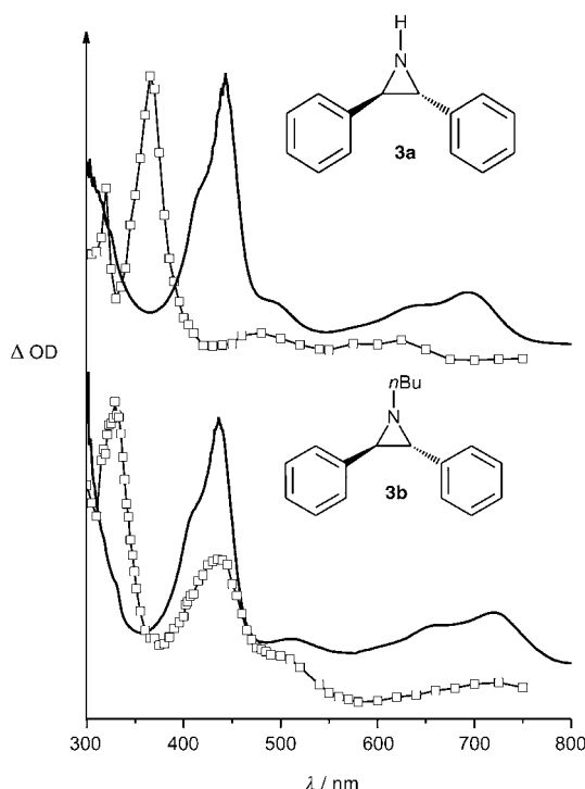
Figure 5. Transient absorption spectra recorded after pulse radiolysis of 8 mM of 3a (□, 2.5 μs) and 9 mM of 3b (□, 2 μs after the electron pulse) in n -butyl chloride and after ^{60}\text{Co} γ radiolysis of the same two 2,3-diphenylaziridines in a Freon matrix at 77 K (—).
